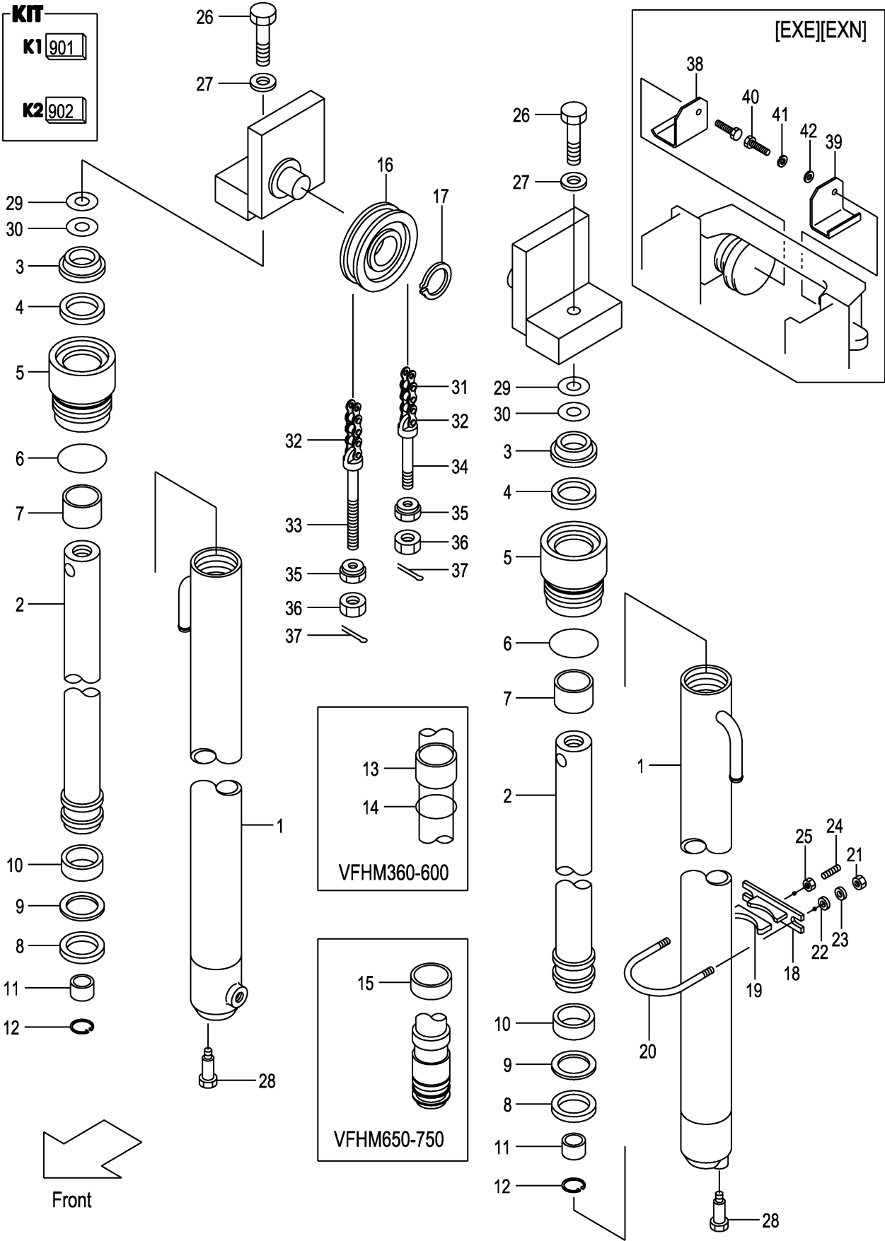
FIG.204 LIFT CYLINDER (REAR)[VFHM0A7] (M7010820) リフトシリンダ
