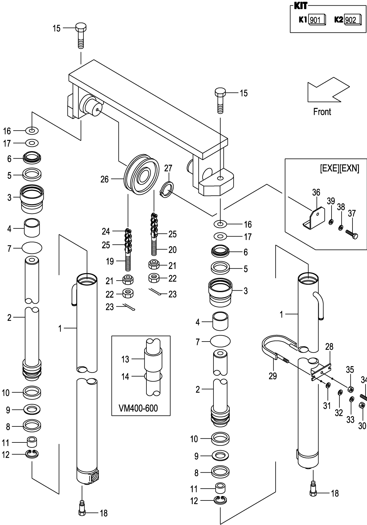
FIG.190 LIFT CYLINDER [VM0A7,VM0A9] (M7018410) リフトシリンダ
