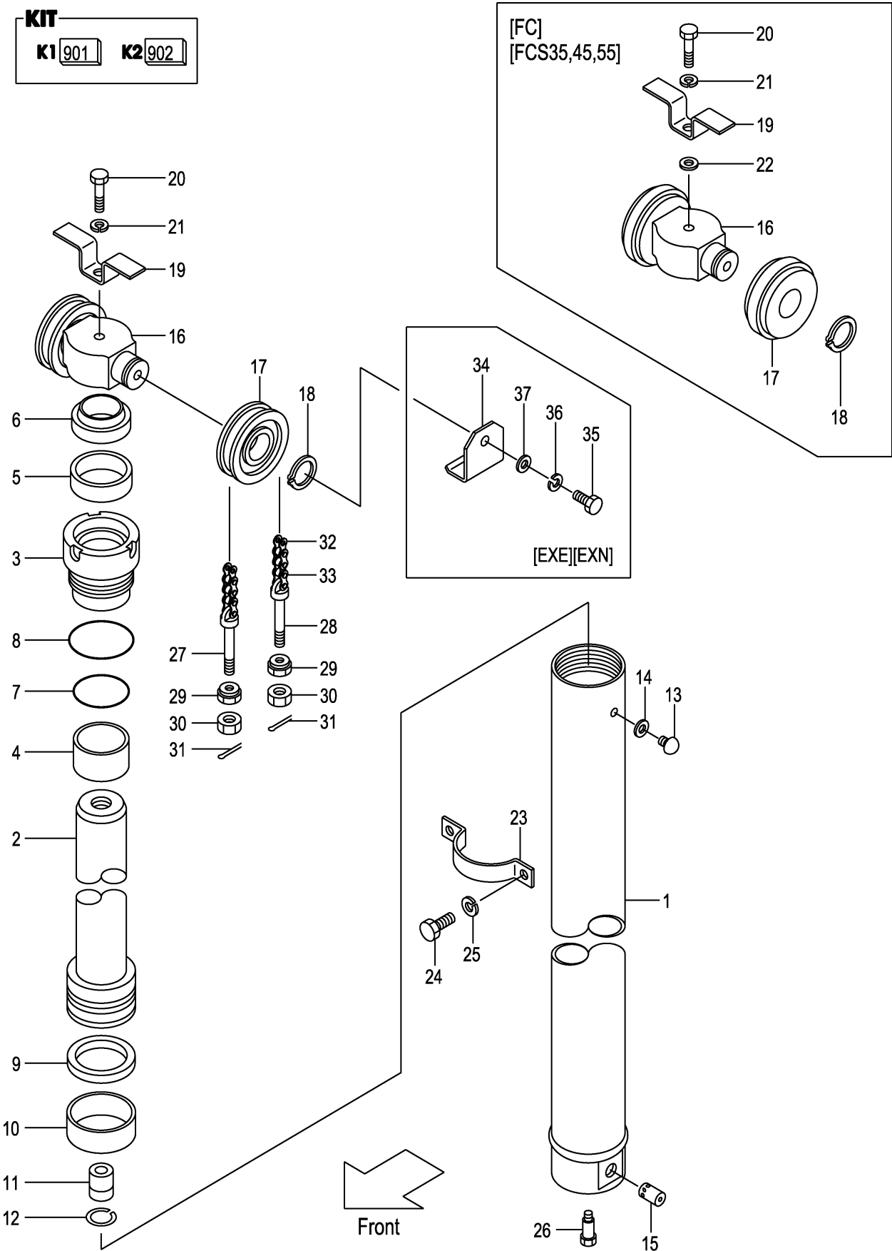
FIG.203 LIFT CYLINDER (FRONT)[VFHM0A7] (M7010810) リフトシリンダ
