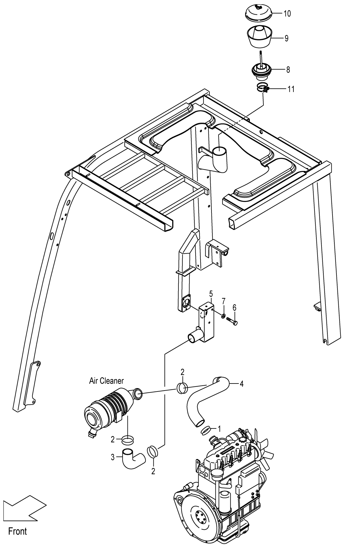
FIG.4 AIR DUCT [CAKB] (F7Z11080) エアダクト
