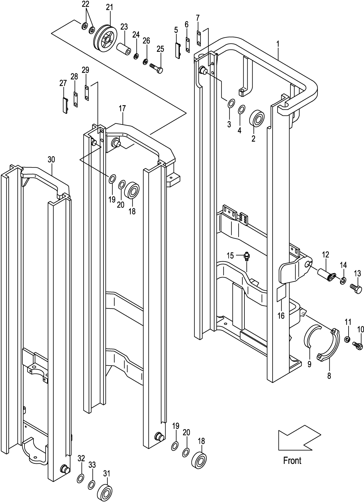
FIG.202 MAST [VFHM0A7] (M7010710) マスト
